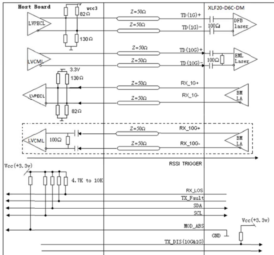
Figure 5 Typical Interface Circuit
