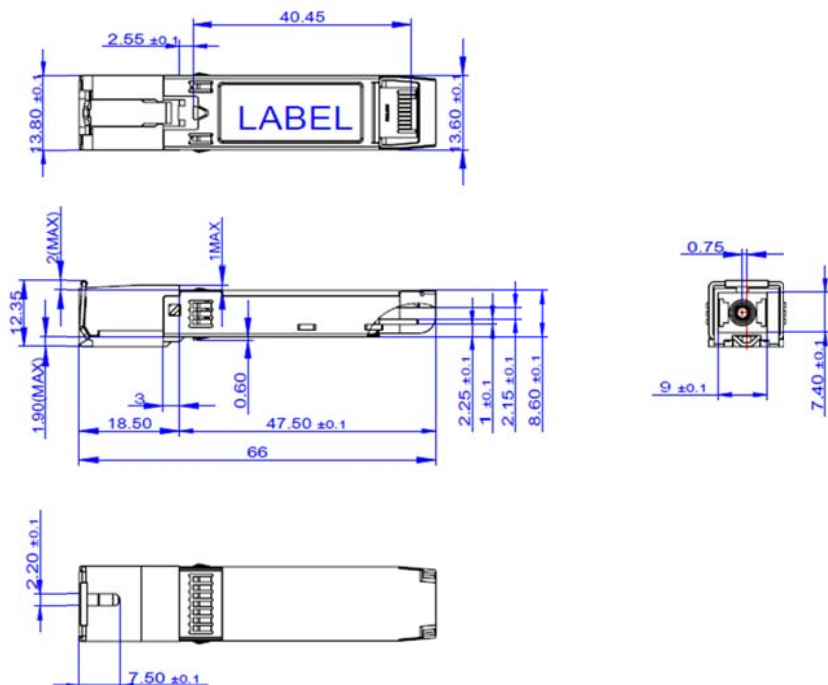
Figure 7 Package Outline
